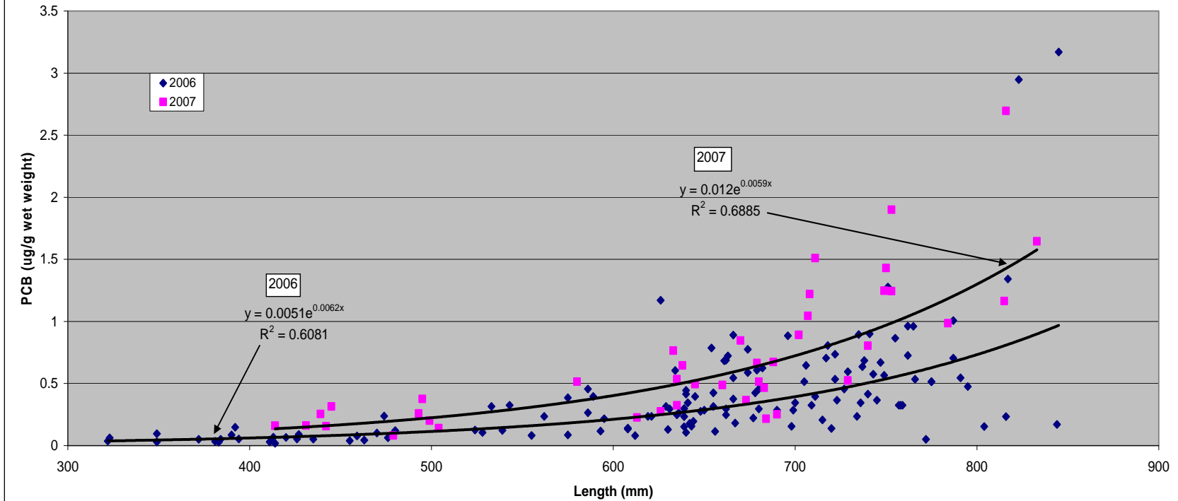
Figure 5: Length-total PCB relationships in bluefish taken from Long Island Sound
