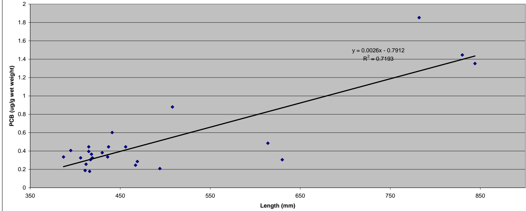
Figure 6: Length-total PCB relationship in weakfish taken from Long Island Sound in 2007
