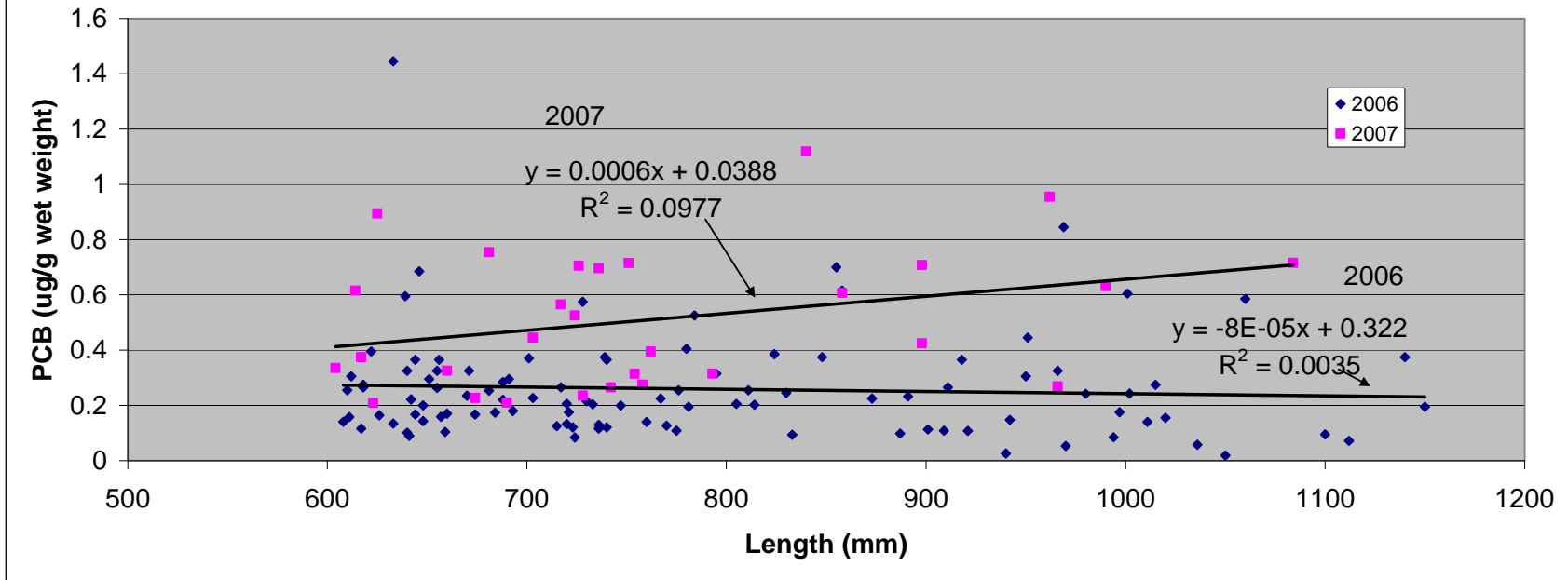
Figure 4: Length-total PCB relationships in striped bass taken from Long Island Sound
