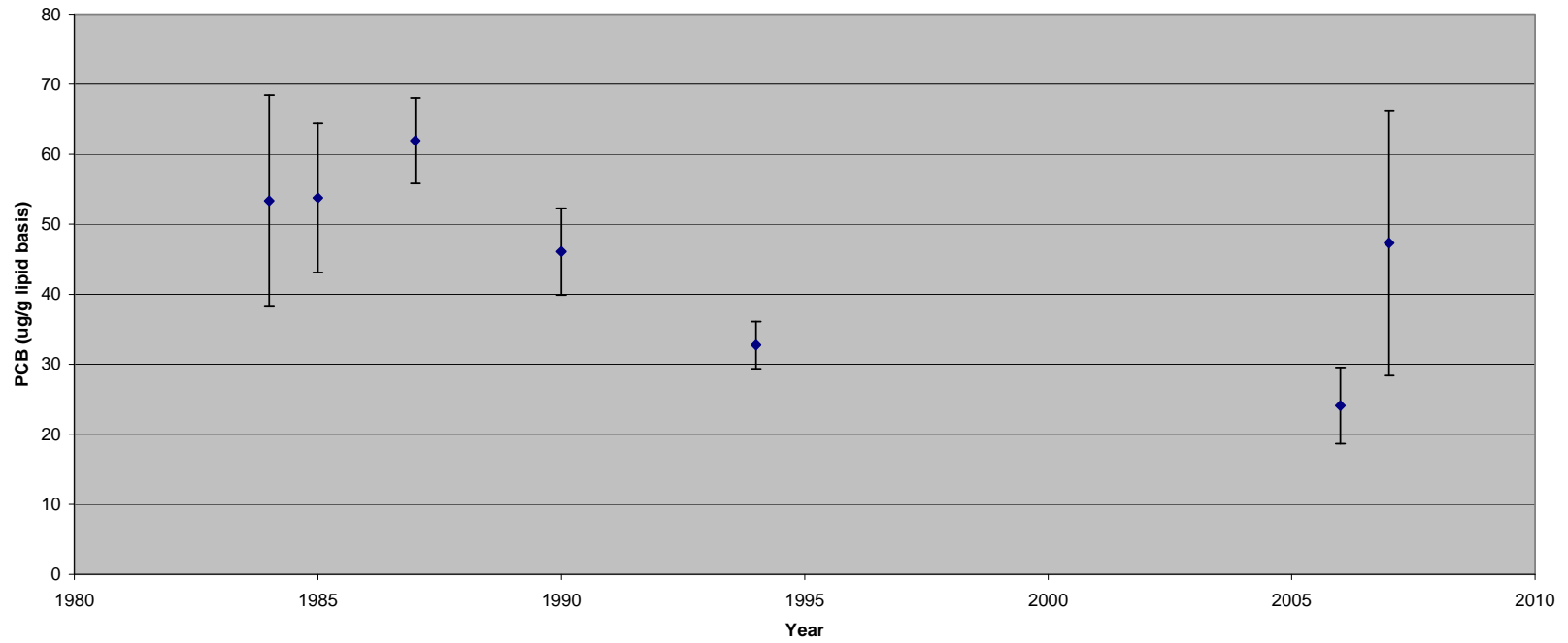
Figure 14: Temporal changes in total PCBs (lipid basis) in striped bass taken from Long Island Sound
