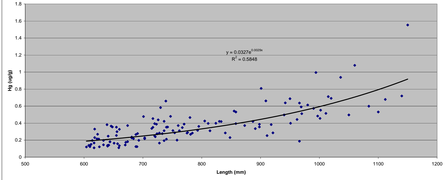
Figure 7: Length-mercury relationship in striped bass taken from Long Island Sound (2006 and 2007 combined)
