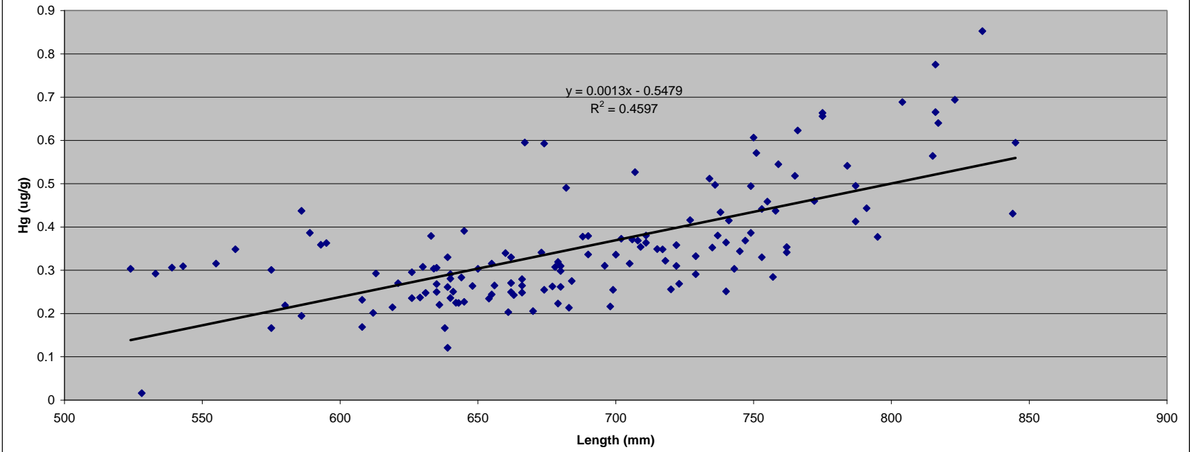
Figure 8: Length-mercury relationship in bluefish greater than 508 mm taken from Long Island Sound (2006 and 2007 combined)
