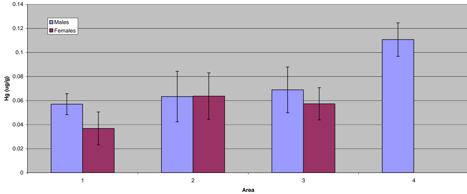
Figure 10: Mercury concentrations by area and sex in hepatopancreas of American lobster taken from Long Island Sound in 2007
