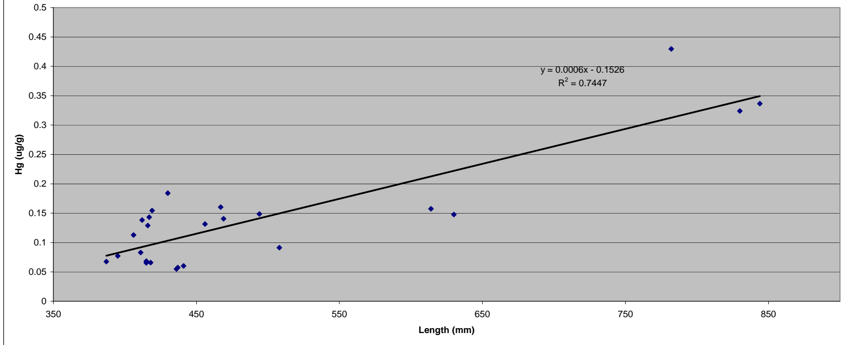
Figure 9: Length-mercury relationship in weakfish taken from Long Island Sound in 2007
