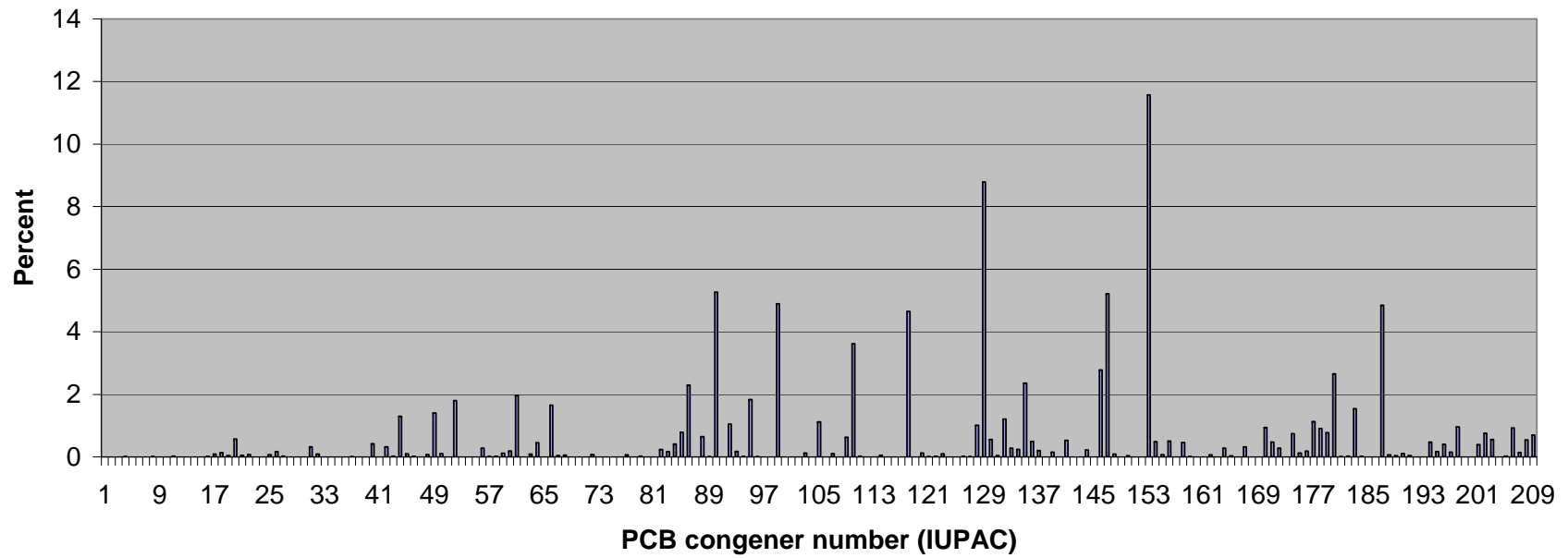
Figure 11: Contributions by PCB congener to total PCB in bluefish taken from Long Island Sound
