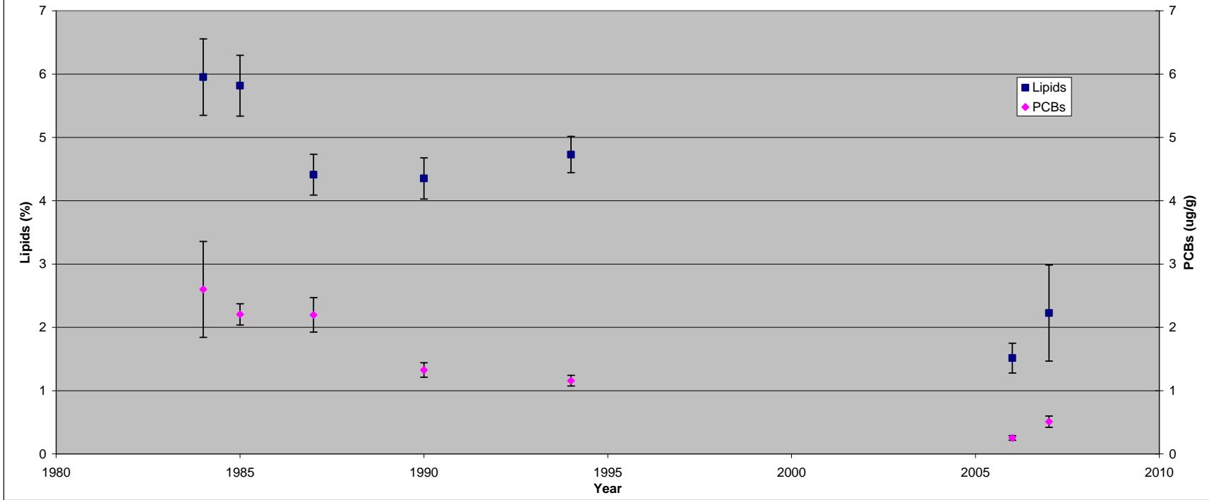
Figure 13: Temporal changes in lipid and PCB concentrations in striped bass from Long Island Sound
