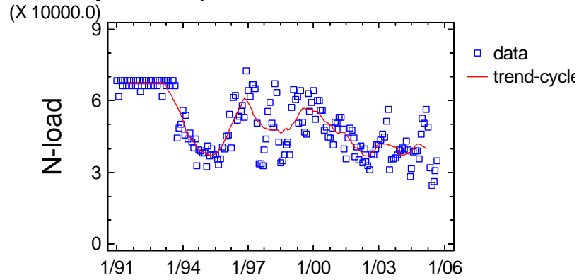
Trend-Cycle Component Plot for Coastal_STPs_6
