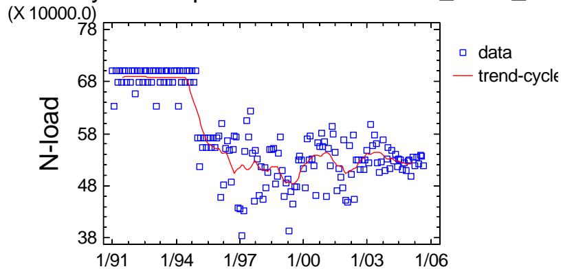
Trend-Cycle Component Plot for Coastal_STPs_9
