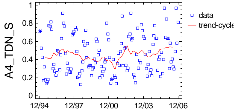
Trend-Cycle Component Plot for A4_TDN_S
