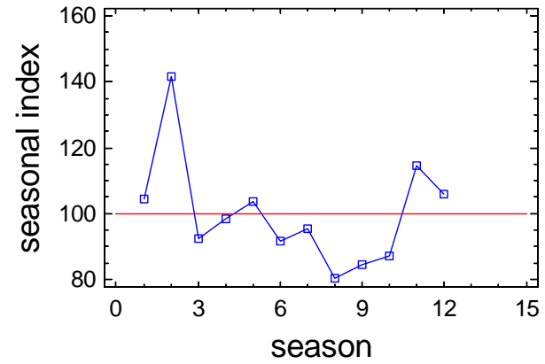
Seasonal Index Plot for K2_TDN_S
