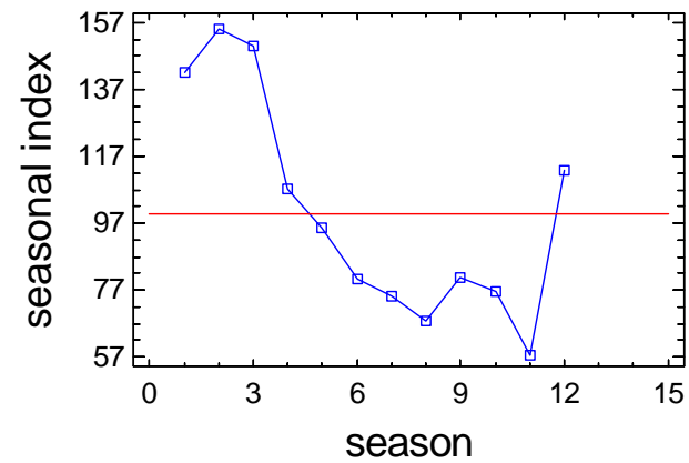
Seasonal Index Plot for F2_CHLA_B
