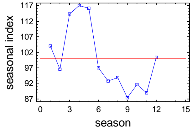
Seasonal Index Plot for Coastal_STPs_4
