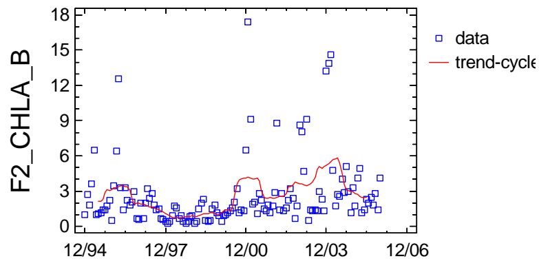
Trend-Cycle Component Plot for F2_CHLA_B
