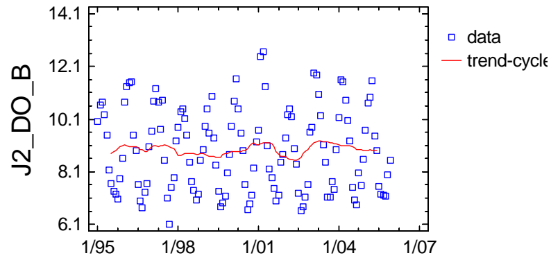
Trend-Cycle Component Plot for J2_DO_B
