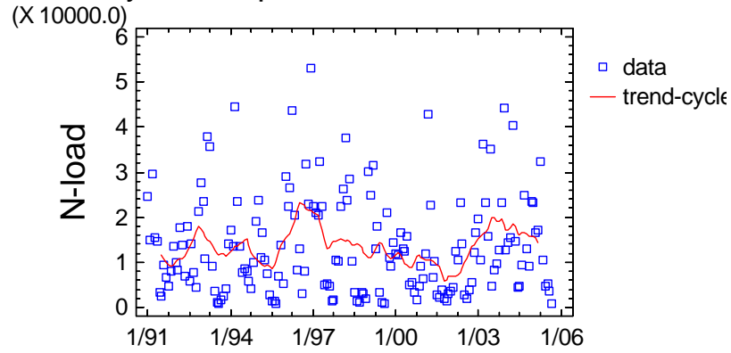
Trend-Cycle Component Plot for Coastal_NPS_7
