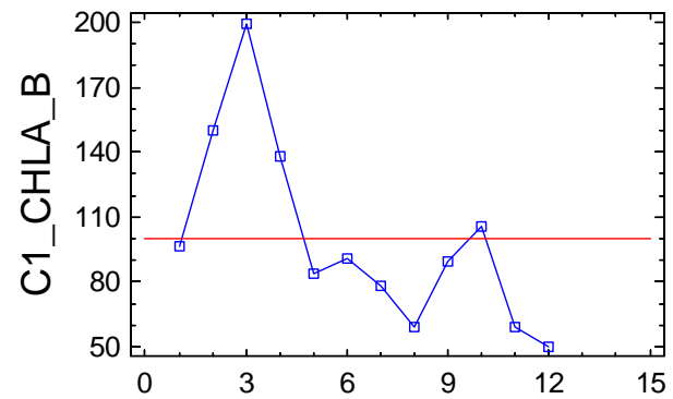
Seasonal Index Plot for C1_CHLA_B
