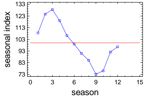
Seasonal Index Plot for H2_DO_S
