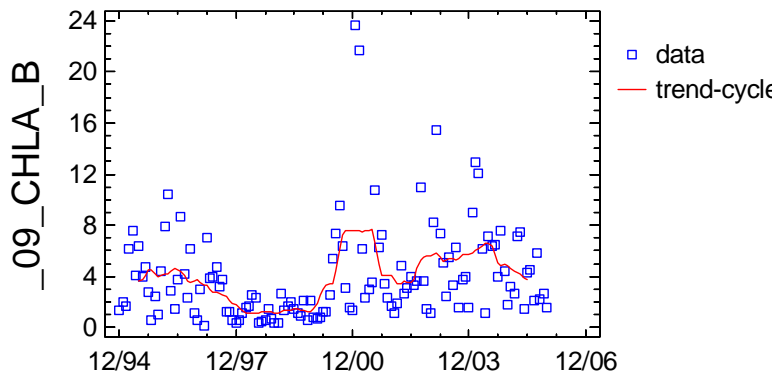
Trend-Cycle Component Plot for _09_CHLA_B
