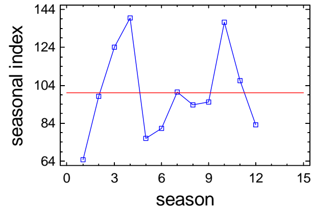
Seasonal Index Plot for J2_CHLA_B
