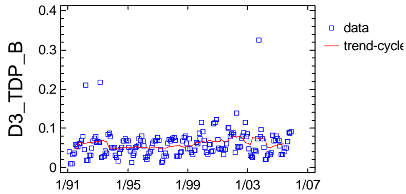
Trend-Cycle Component Plot for D3_TDP_B
