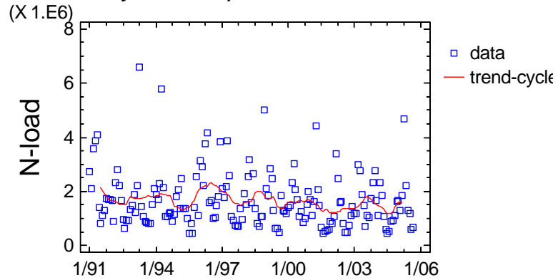
Trend-Cycle Component Plot for Total_2
