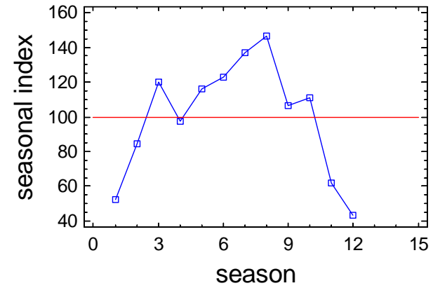
Seasonal Index Plot for C1_CHLA_S
