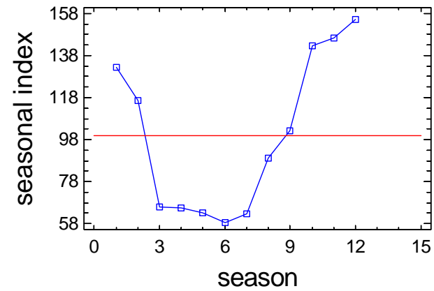
Seasonal Index Plot for _15_TDP_S
