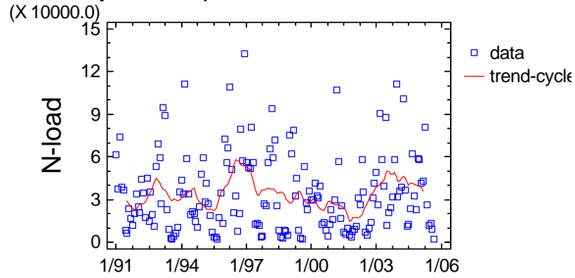
Trend-Cycle Component Plot for Coastal_NPS_5
