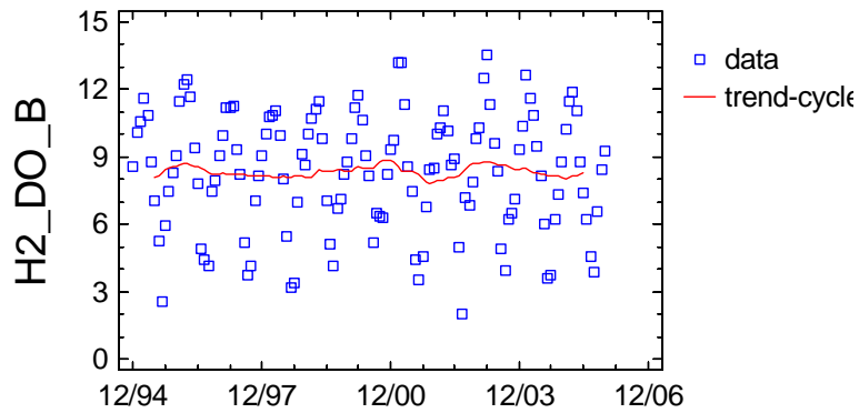
Trend-Cycle Component Plot for H2_DO_B
