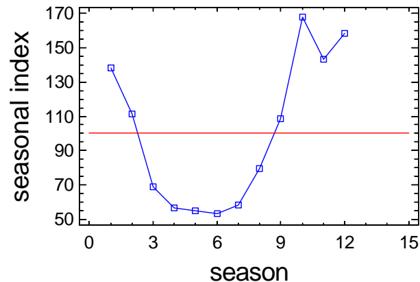
Seasonal Index Plot for C2_TDP_S
