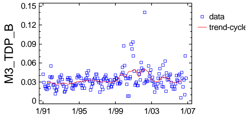
Trend-Cycle Component Plot for M3_TDP_B
