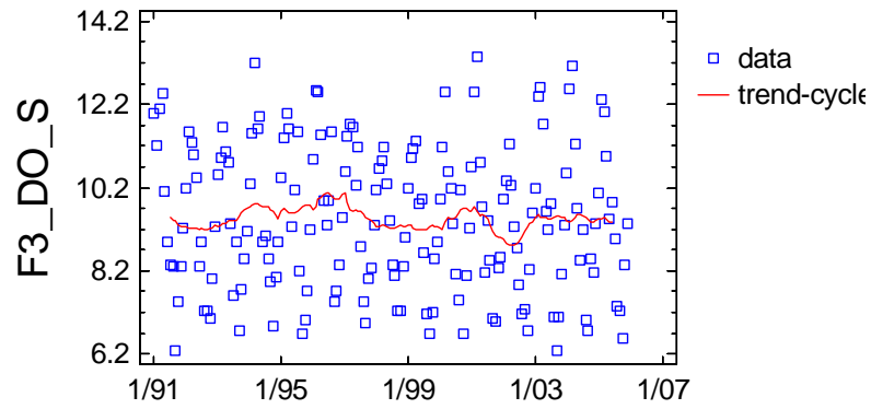
Trend-Cycle Component Plot for F3_DO_S
