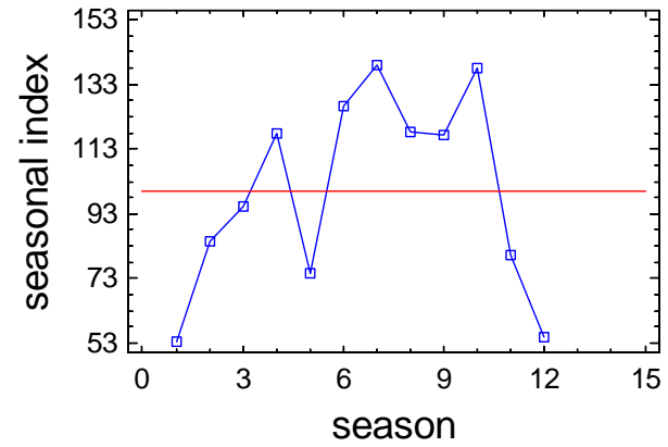
Seasonal Index Plot for K2_CHLA_S
