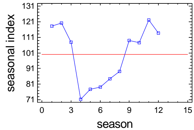
Seasonal Index Plot for D3_TDN_B
