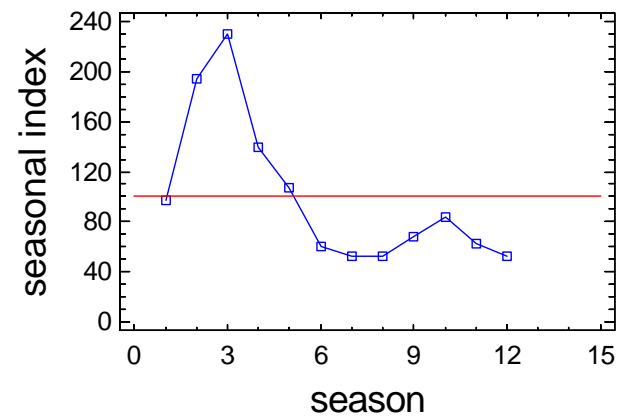
Seasonal Index Plot for D3_CHLA_B
