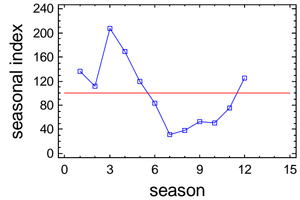
Seasonal Index Plot for Coastal_NPS_7
