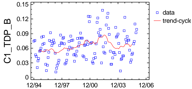
Trend-Cycle Component Plot for C1_TDP_B
