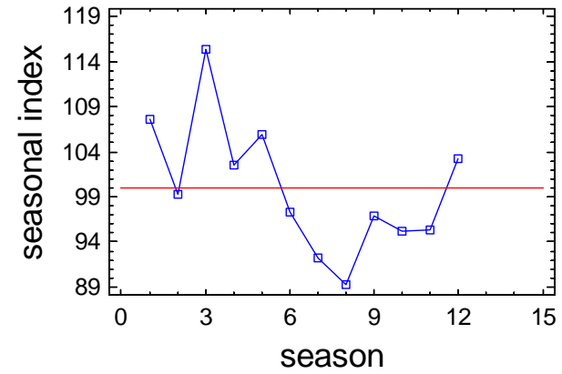
Seasonal Index Plot for Coastal_STPs_1
