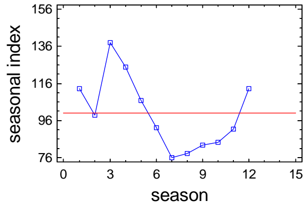
Seasonal Index Plot for Total_10
