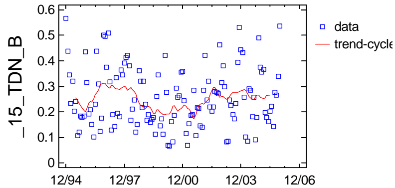
Trend-Cycle Component Plot for _15_TDN_B
