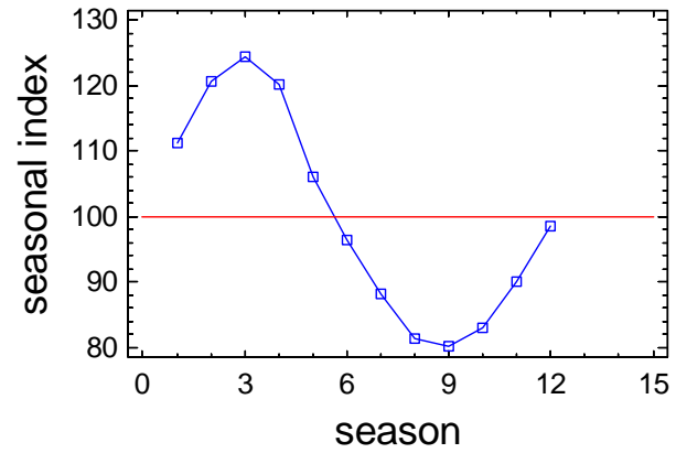
Seasonal Index Plot for K2_DO_S
