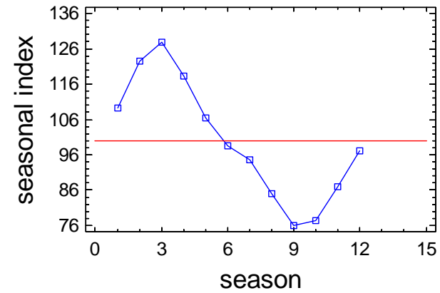
Seasonal Index Plot for F3_DO_S
