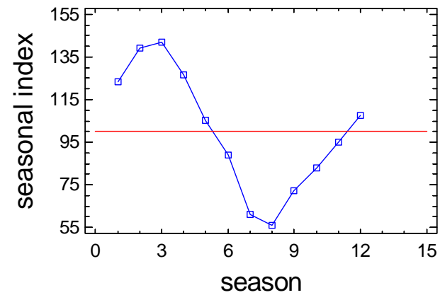
Seasonal Index Plot for _15_DO_B
