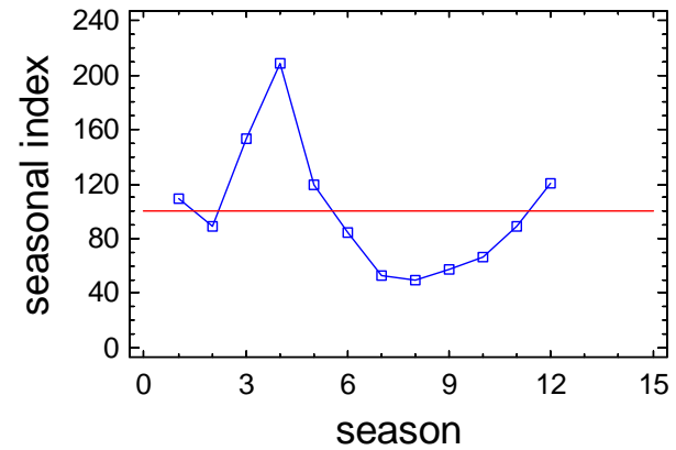
Seasonal Index Plot for Total_2
