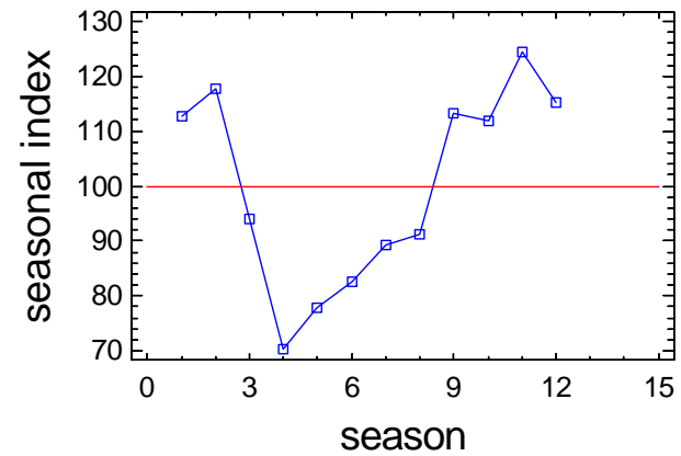
Seasonal Index Plot for C2_TDN_B
