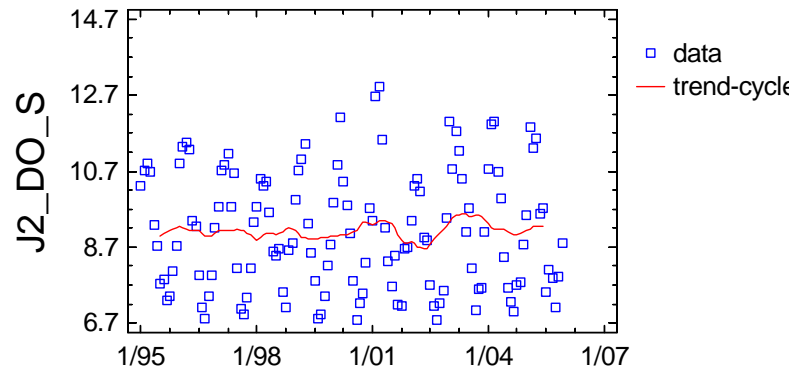
Trend-Cycle Component Plot for J2_DO_S
