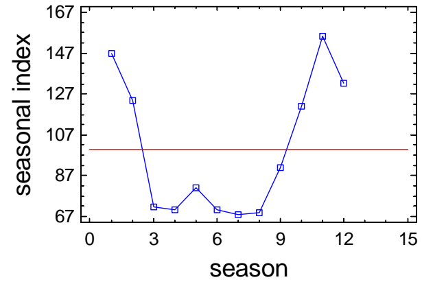
Seasonal Index Plot for B3_TDN_S
