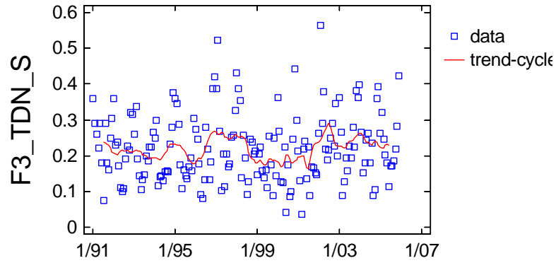
Trend-Cycle Component Plot for F3_TDN_S
