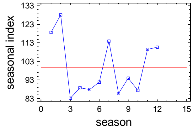
Seasonal Index Plot for K2_TDN_B
