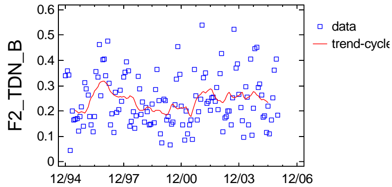
Trend-Cycle Component Plot for F2_TDN_B
