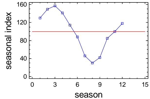
Seasonal Index Plot for B3_DO_B
