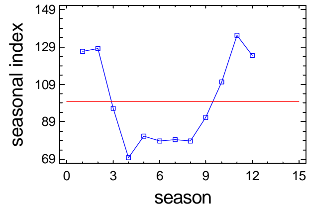
Seasonal Index Plot for D3_TDN_S
