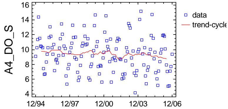
Trend-Cycle Component Plot for A4_DO_S
