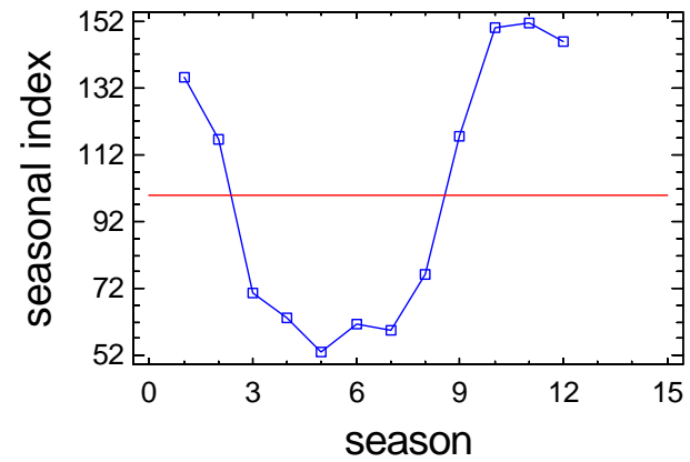
Seasonal Index Plot for D3_TDP_S
