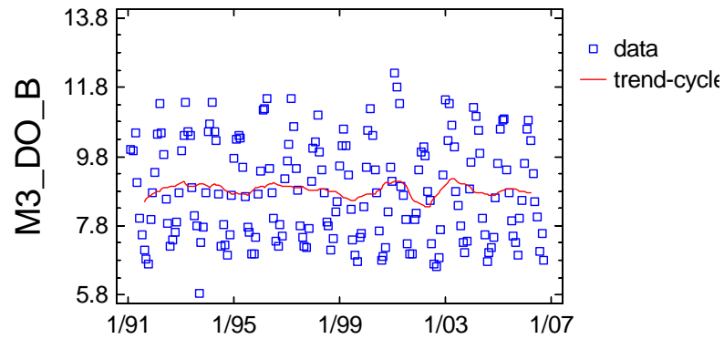
Trend-Cycle Component Plot for M3_DO_B
