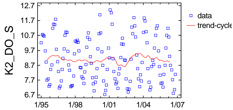
Trend-Cycle Component Plot for K2_DO_S
