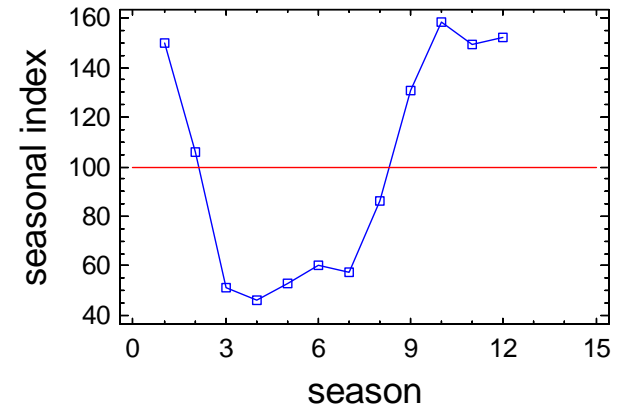
Seasonal Index Plot for B3_TDP_S
