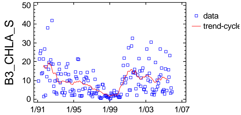
Trend-Cycle Component Plot for B3_CHLA_S
