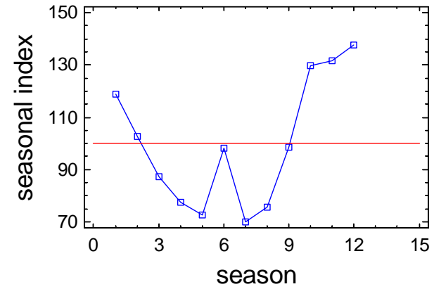
Seasonal Index Plot for K2_TDP_S
