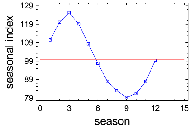
Seasonal Index Plot for M3_DO_B
