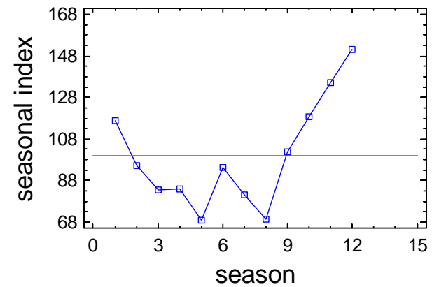
Seasonal Index Plot for K2_TDP_B
