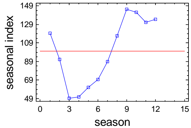
Seasonal Index Plot for A4_TDP_B
