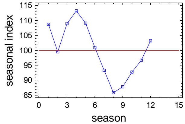
Seasonal Index Plot for Coastal_STPs_2
