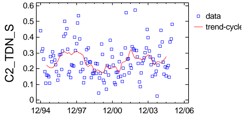
Trend-Cycle Component Plot for C2_TDN_S
