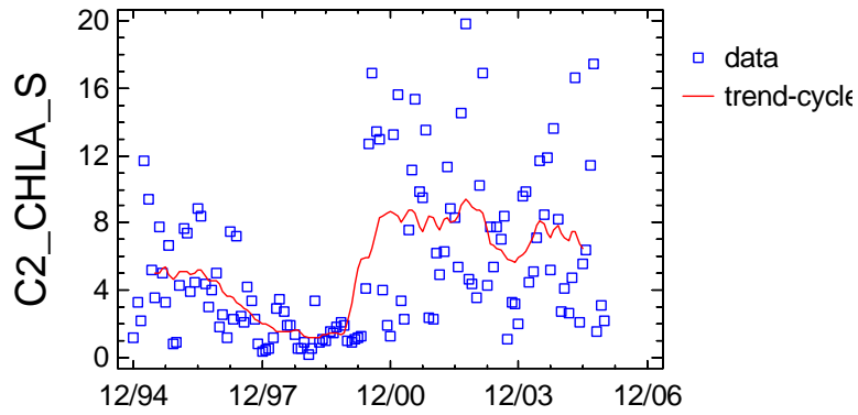
Trend-Cycle Component Plot for C2_CHLA_S
