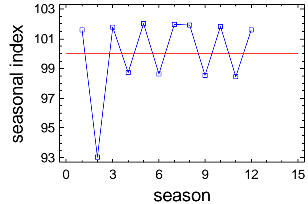
Seasonal Index Plot for Coastal_STPs_7
