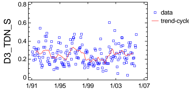
Trend-Cycle Component Plot for D3_TDN_S
