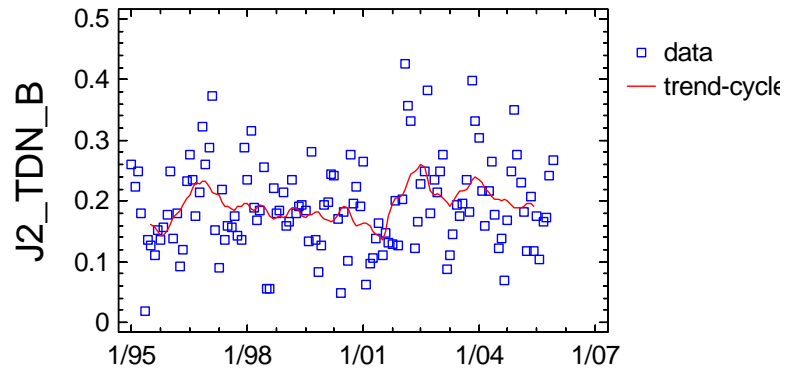
Trend-Cycle Component Plot for J2_TDN_B
