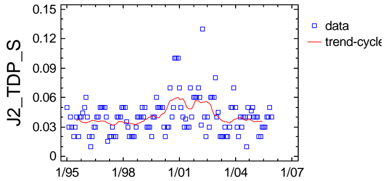
Trend-Cycle Component Plot for J2_TDP_S
