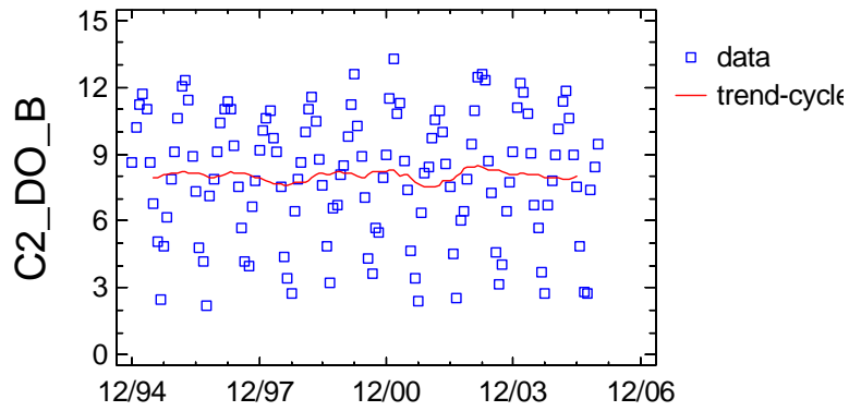
Trend-Cycle Component Plot for C2_DO_B
