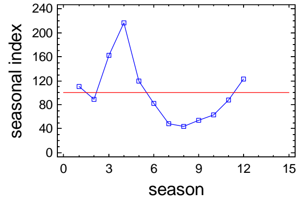
Seasonal Index Plot for Tributaries_2
