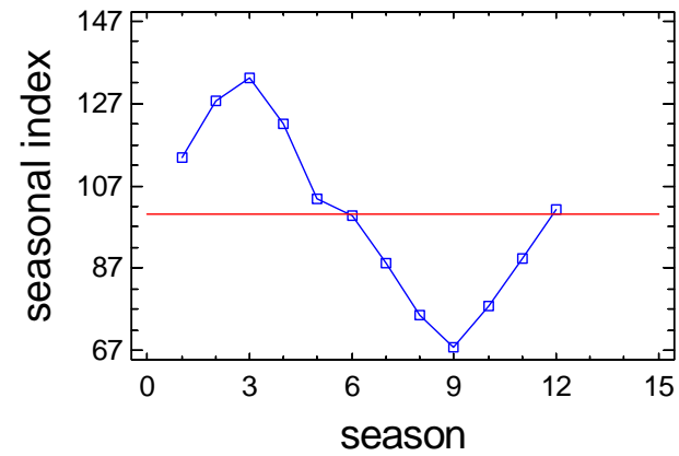
Seasonal Index Plot for F2_DO_S
