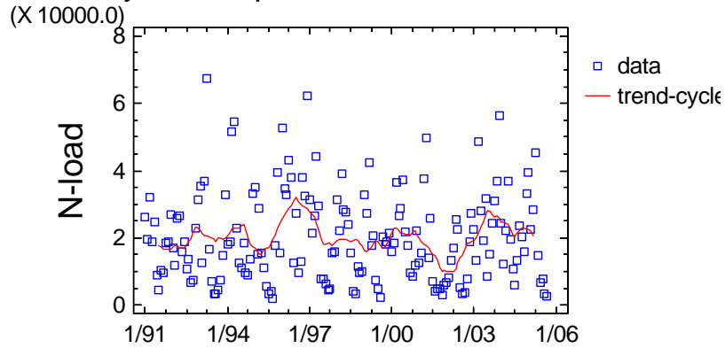
Trend-Cycle Component Plot for Coastal_NPS_4
