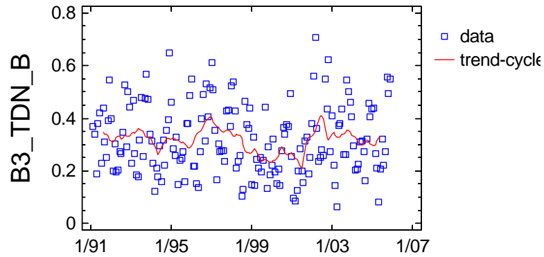
Trend-Cycle Component Plot for B3_TDN_B
