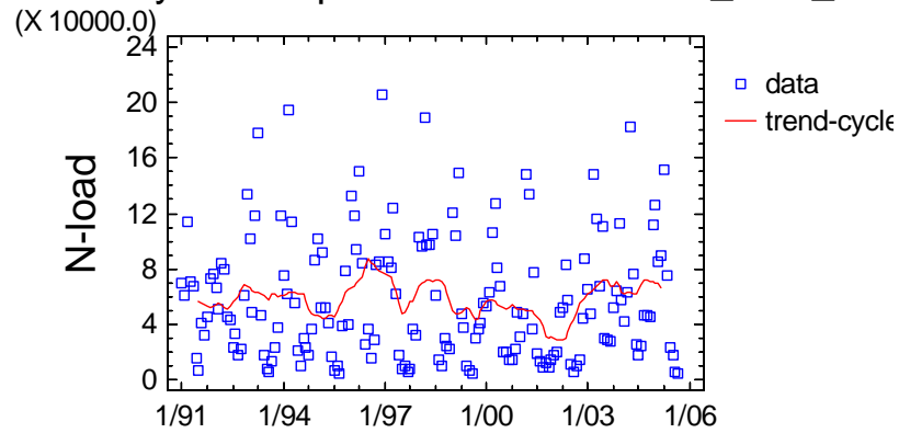
Trend-Cycle Component Plot for Coastal_NPS_1
