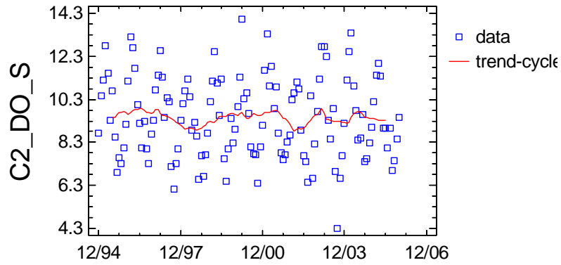
Trend-Cycle Component Plot for C2_DO_S
