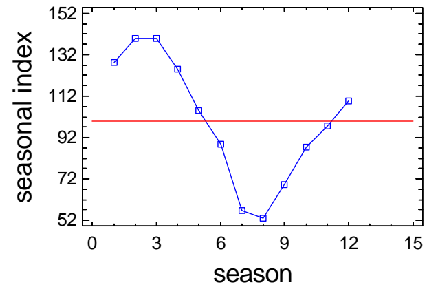
Seasonal Index Plot for _09_DO_B
