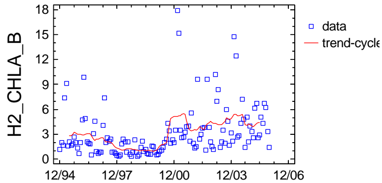
Trend-Cycle Component Plot for H2_CHLA_B
