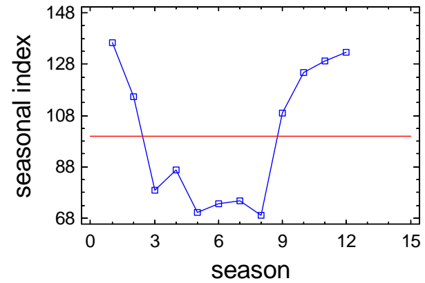
Seasonal Index Plot for J2_TDP_B
