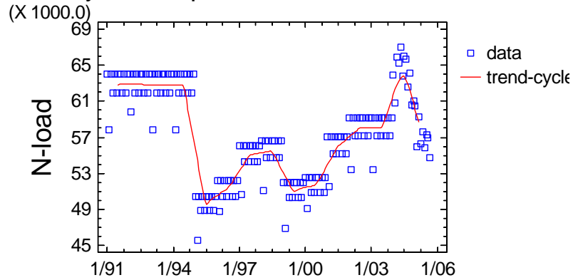
Trend-Cycle Component Plot for Coastal_STPs_7
