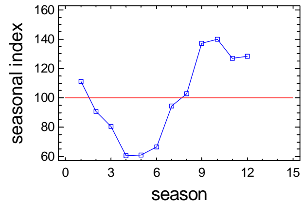
Seasonal Index Plot for F2_TDP_B
