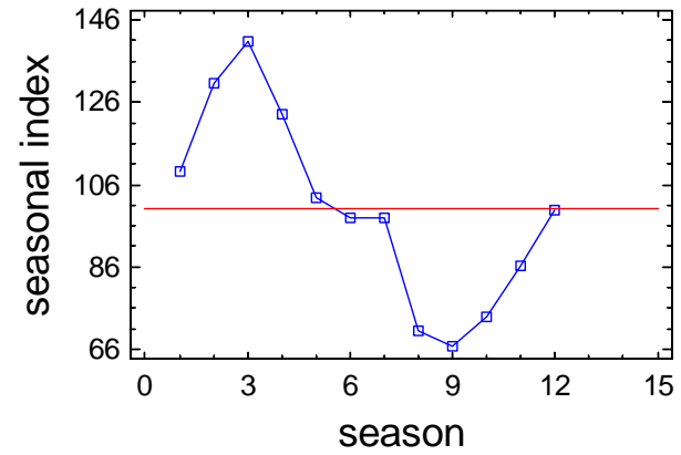
Seasonal Index Plot for A4_DO_S
