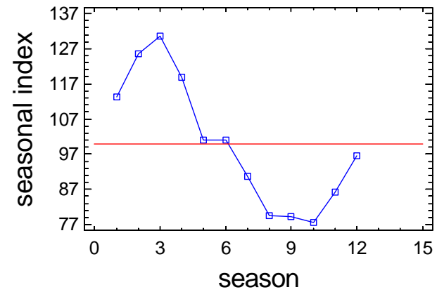
Seasonal Index Plot for C2_DO_S
