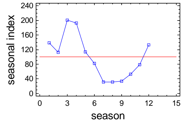
Seasonal Index Plot for Coastal_NPS_1
