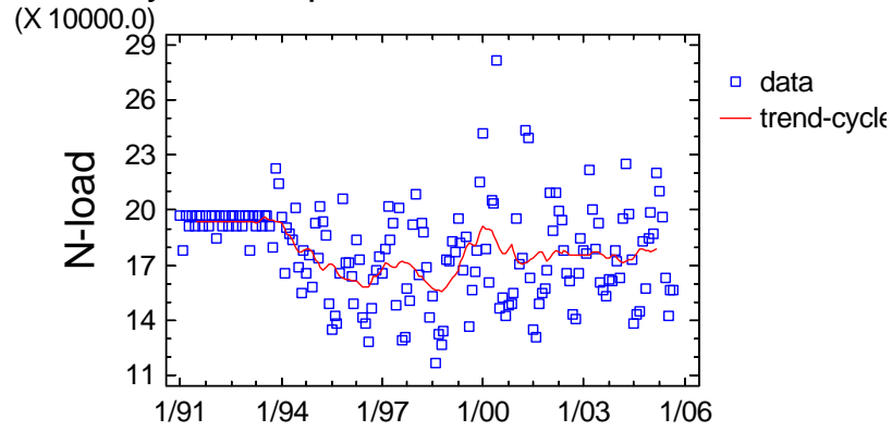
Trend-Cycle Component Plot for Coastal_STPs_2
