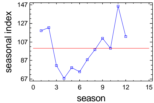
Seasonal Index Plot for _09_TDN_B
