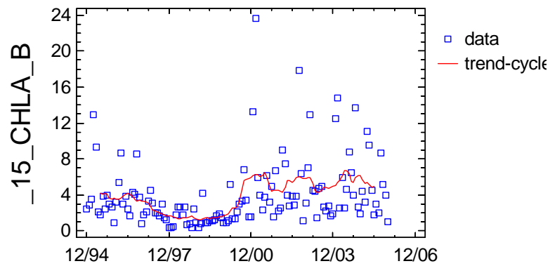
Trend-Cycle Component Plot for _15_CHLA_B
