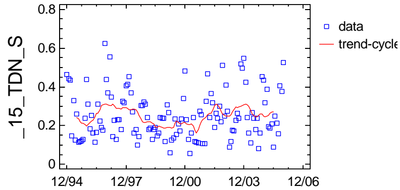
Trend-Cycle Component Plot for _15_TDN_S
