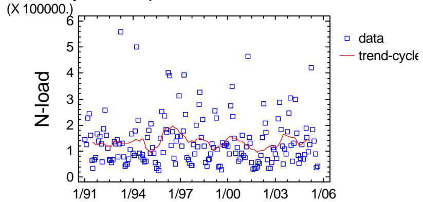
Trend-Cycle Component Plot for Coastal_NPS_2
