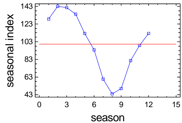
Seasonal Index Plot for D3_DO_B
