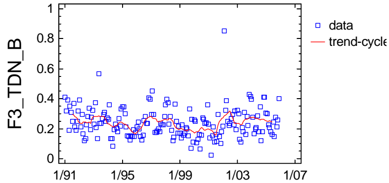
Trend-Cycle Component Plot for F3_TDN_B
