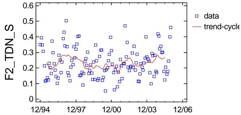
Trend-Cycle Component Plot for F2_TDN_S
