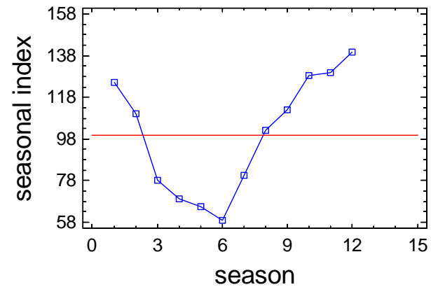
Seasonal Index Plot for F3_TDP_B
