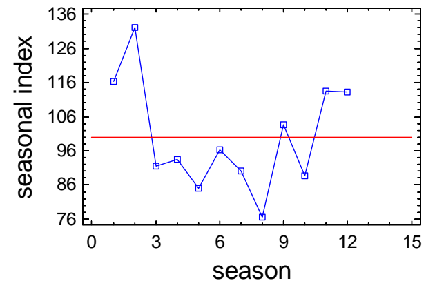
Seasonal Index Plot for M3_TDN_B
