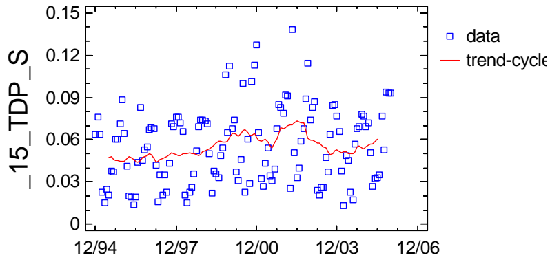
Trend-Cycle Component Plot for _15_TDP_S
