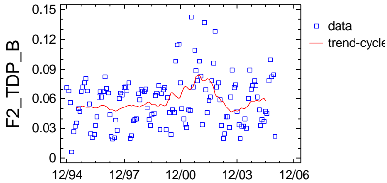
Trend-Cycle Component Plot for F2_TDP_B
