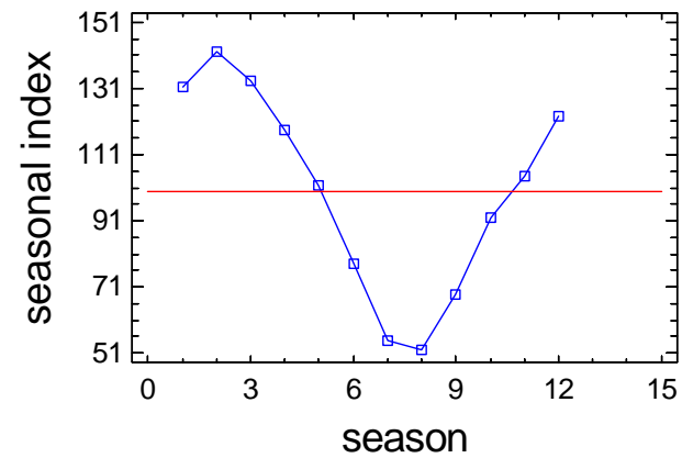
Seasonal Index Plot for F2_DO_B
