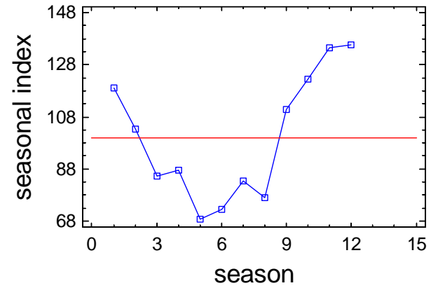
Seasonal Index Plot for M3_TDP_S
