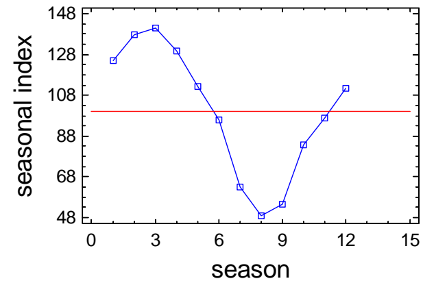
Seasonal Index Plot for F3_DO_B
