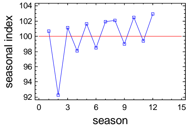
Seasonal Index Plot for Coastal_STPs_10
