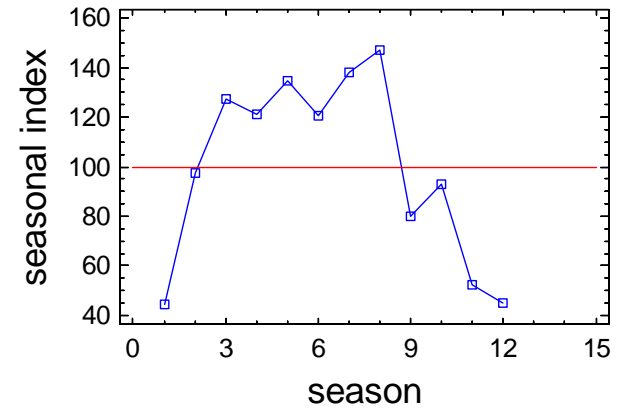
Seasonal Index Plot for B3_CHLA_S
