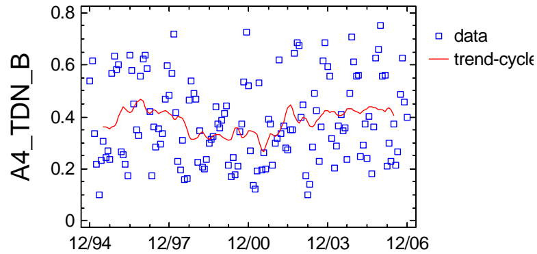
Trend-Cycle Component Plot for A4_TDN_B
