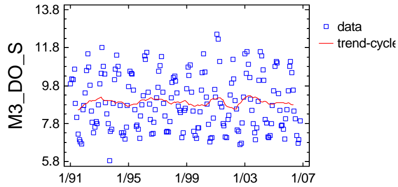
Trend-Cycle Component Plot for M3_DO_S
