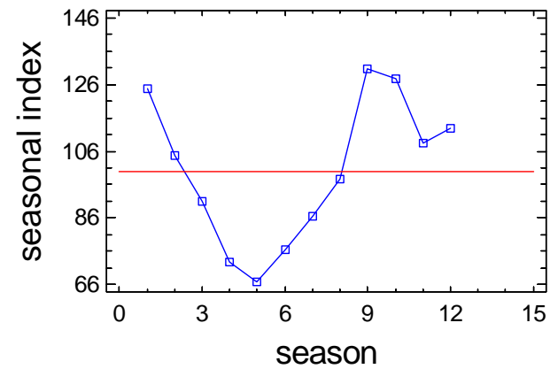
Seasonal Index Plot for F2_TDN_B
