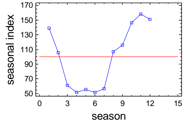
Seasonal Index Plot for C1_TDP_S
