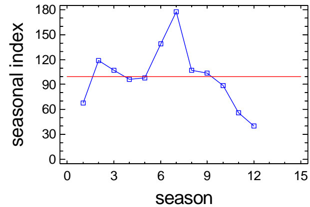
Seasonal Index Plot for F2_CHLA_S
