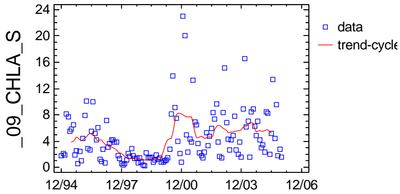
Trend-Cycle Component Plot for _09_CHLA_S
