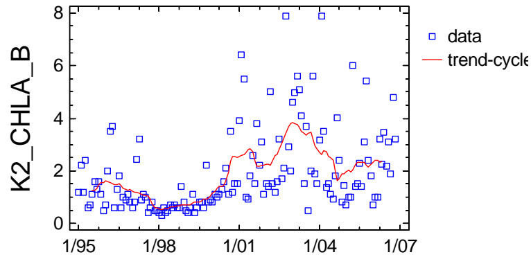
Trend-Cycle Component Plot for K2_CHLA_B
