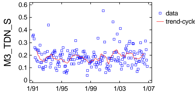
Trend-Cycle Component Plot for M3_TDN_S
