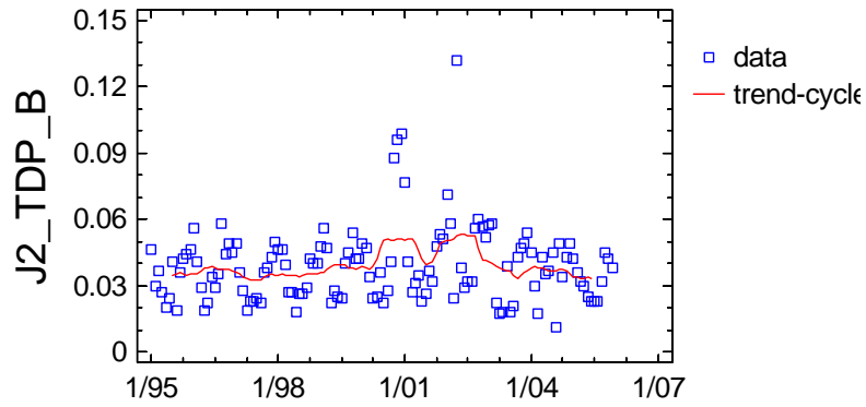
Trend-Cycle Component Plot for J2_TDP_B
