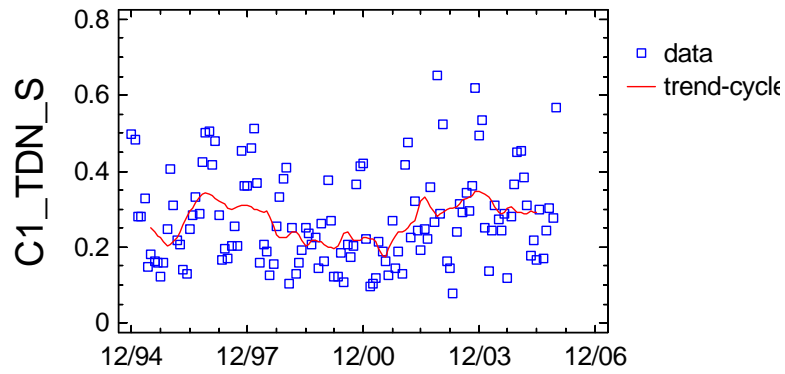
Trend-Cycle Component Plot for C1_TDN_S
