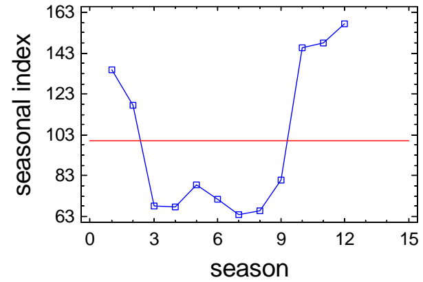
Seasonal Index Plot for A4_TDN_S
