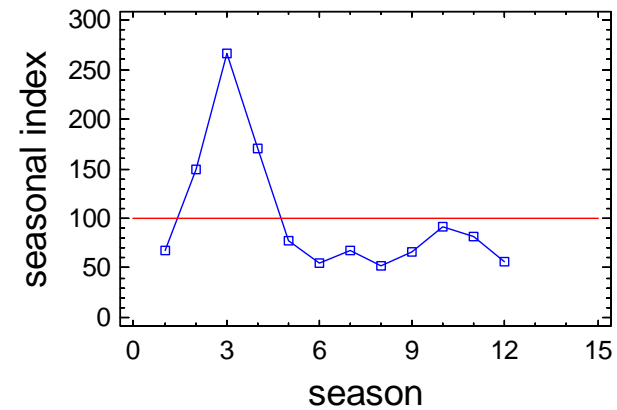
Seasonal Index Plot for F3_CHLA_B
