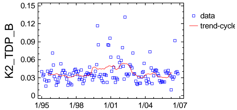
Trend-Cycle Component Plot for K2_TDP_B
