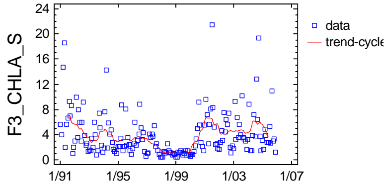
Trend-Cycle Component Plot for F3_CHLA_S
