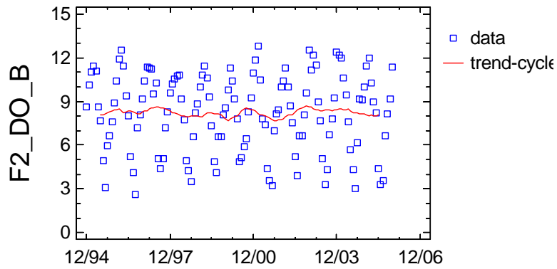
Trend-Cycle Component Plot for F2_DO_B
