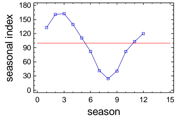
Seasonal Index Plot for A4_DO_B
