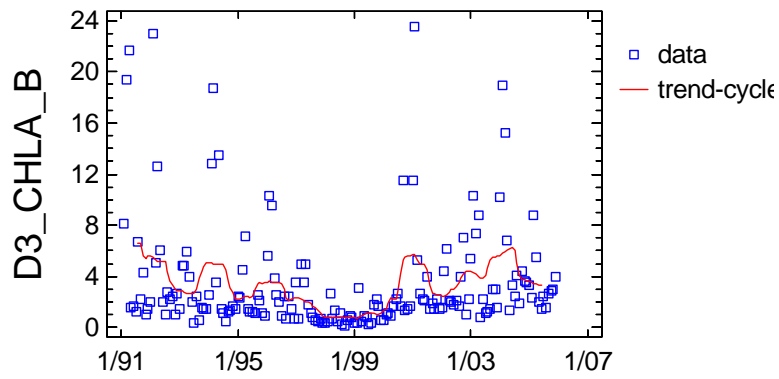
Trend-Cycle Component Plot for D3_CHLA_B
