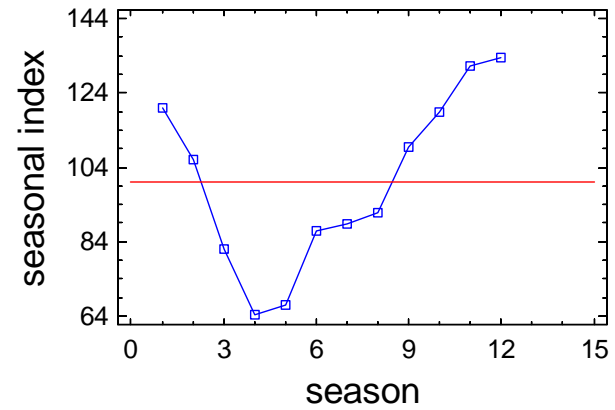
Seasonal Index Plot for B3_TDN_B
