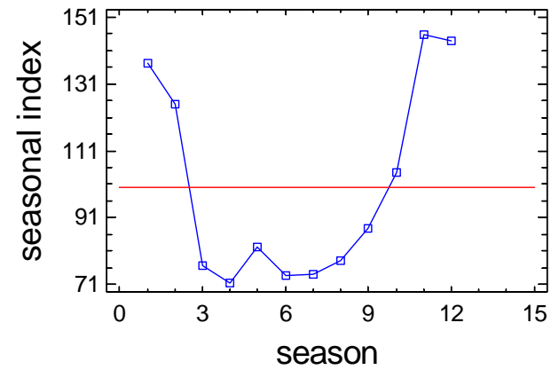
Seasonal Index Plot for _15_TDN_S
