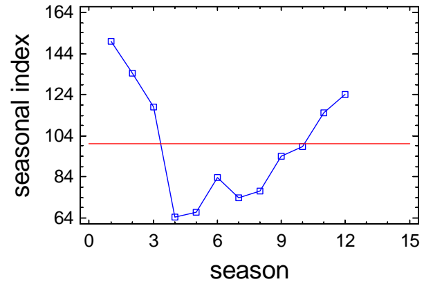
Seasonal Index Plot for H2_TDN_S
