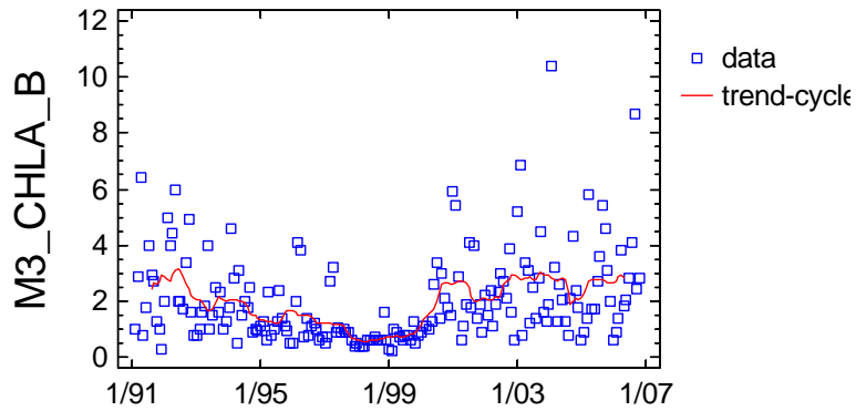
Trend-Cycle Component Plot for M3_CHLA_B
