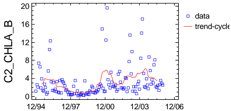
Trend-Cycle Component Plot for C2_CHLA_B
