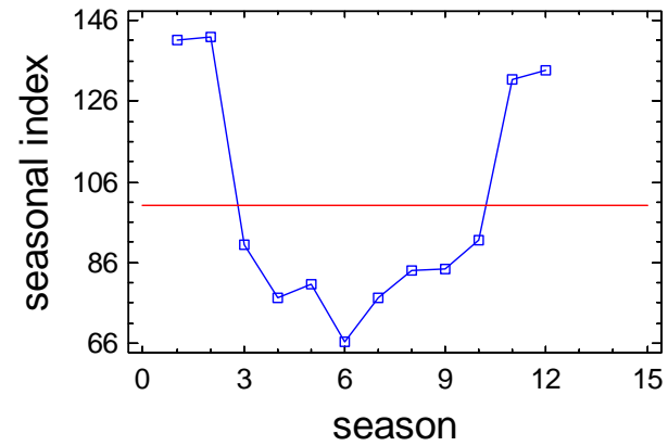
Seasonal Index Plot for F3_TDN_S
