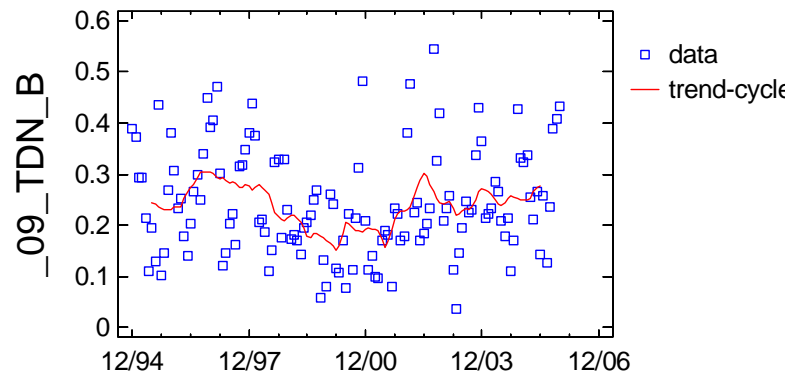
Trend-Cycle Component Plot for _09_TDN_B
