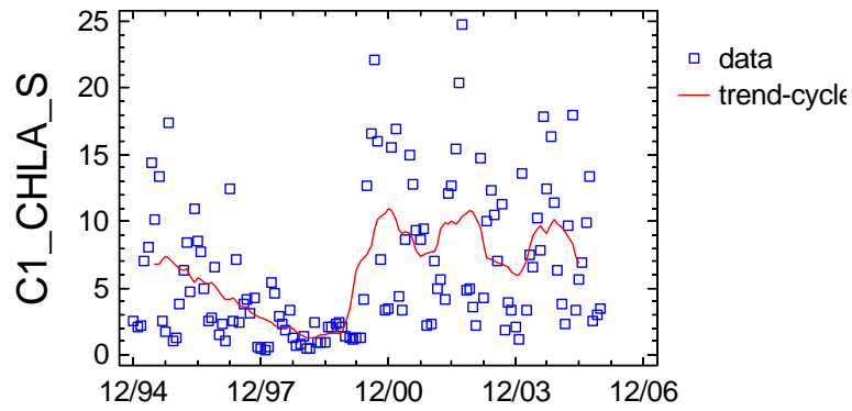
Trend-Cycle Component Plot for C1_CHLA_S
