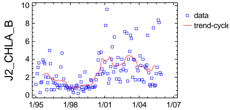
Trend-Cycle Component Plot for J2_CHLA_B
