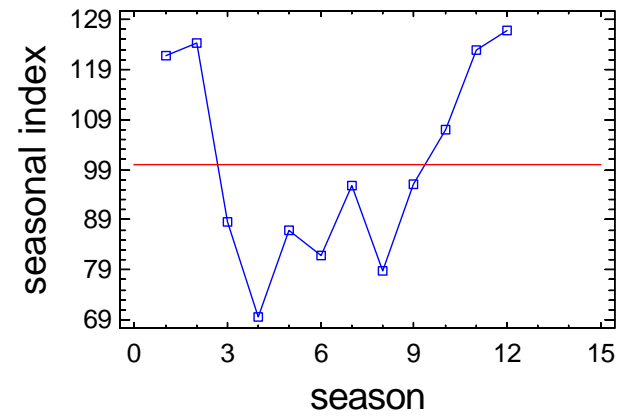
Seasonal Index Plot for _09_TDN_S
