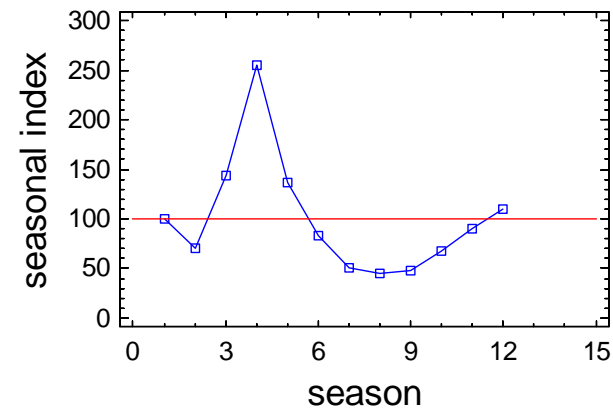
Seasonal Index Plot for Coastal_NPS_2
